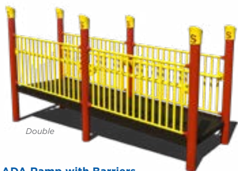
ADA Ramp with Barriers Available for 5" posts 6' or 12' length Available as single or double (pictured) width
